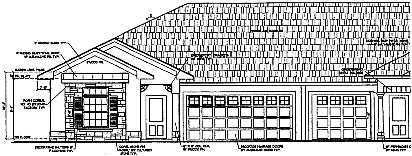
1 FRONT ELEVATION 2
